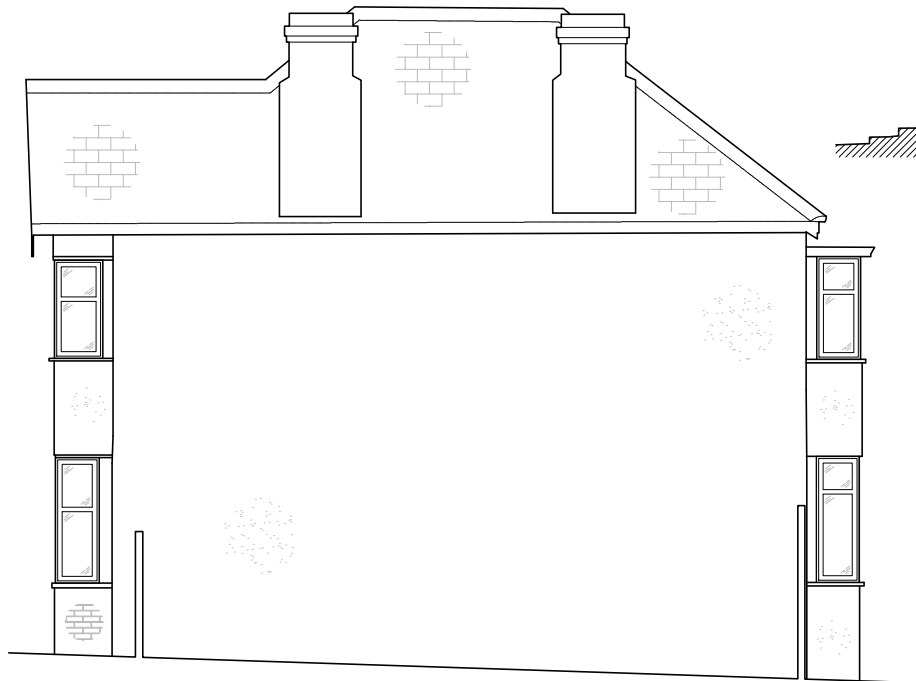
EXISTING RIGHT ELEVATION SCALE 1:100
