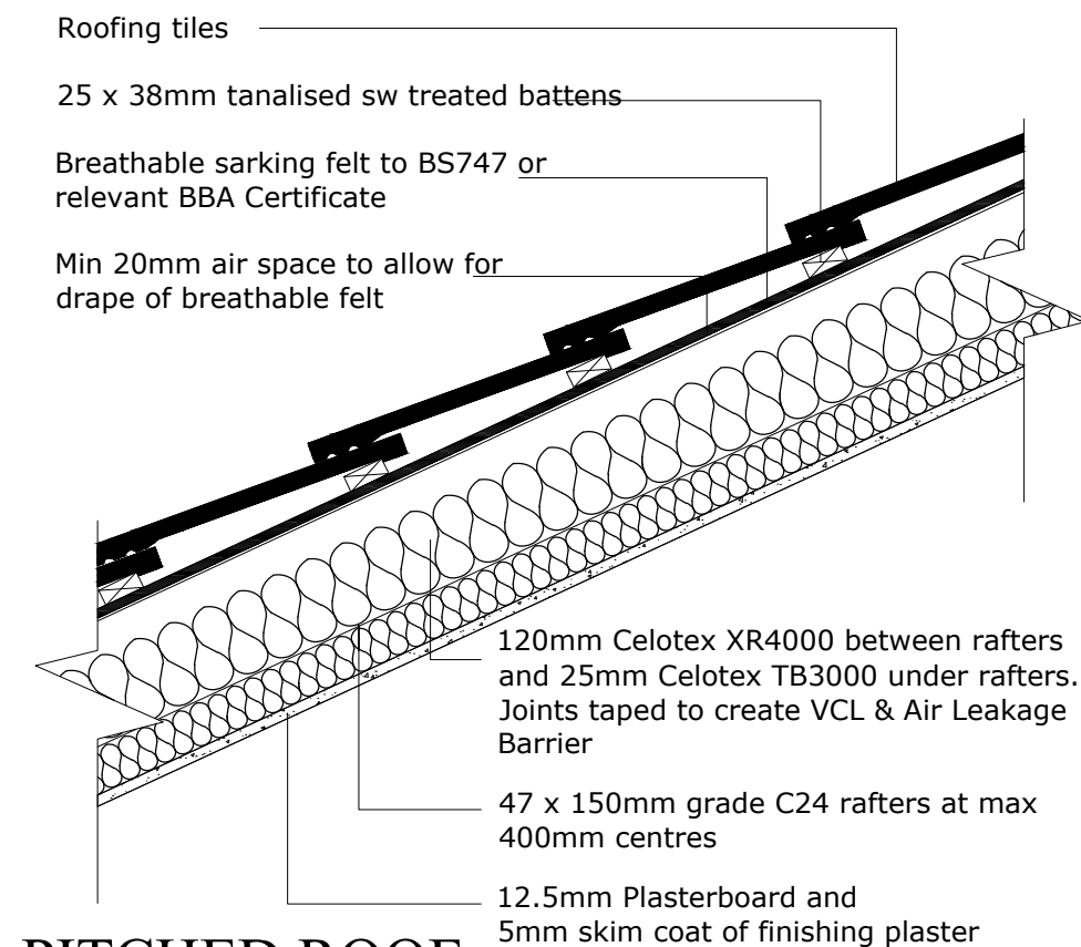
PITCHED ROOF
